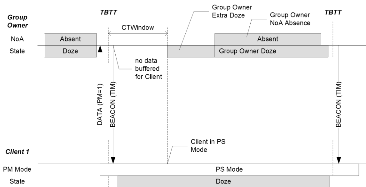
Figure 16—P2P Group Owner Notice of Absence with Opportunistic Power Save
