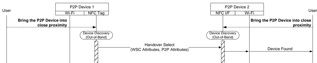
Figure 8—Out-of-Band Device Discovery (NFC Static Handover)
