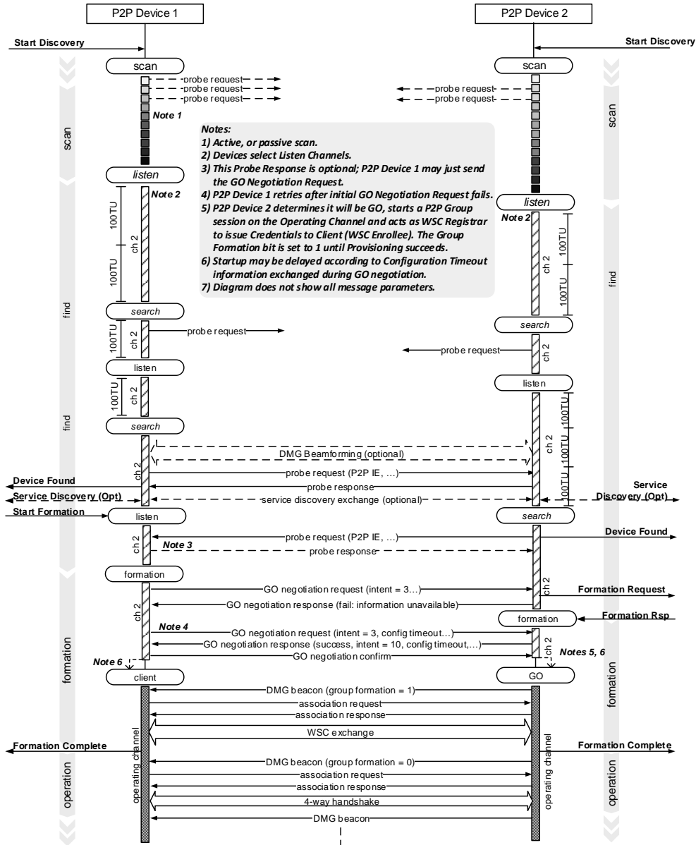
Scenario 1a within DMG: Two P2P Devices discovering each other; group formation occurs on Listen Channel of P2P Device 1
