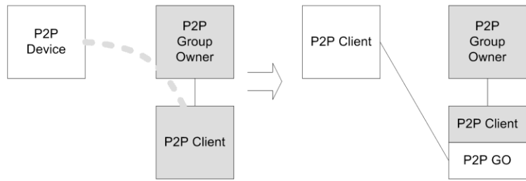
Scenario 4: P2P Device discovering a P2P Device that is the Client in an existing P2P Group and requesting device to reinvok a Persistent P2P Group
